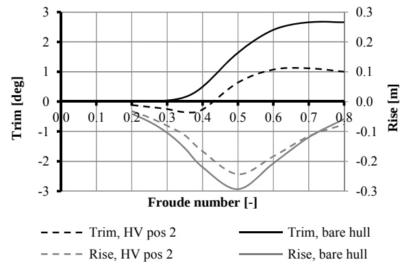
Figure 4. Trim and rise of the bare hull geometry, and the geometry with Hull Vane ® in position 2.
